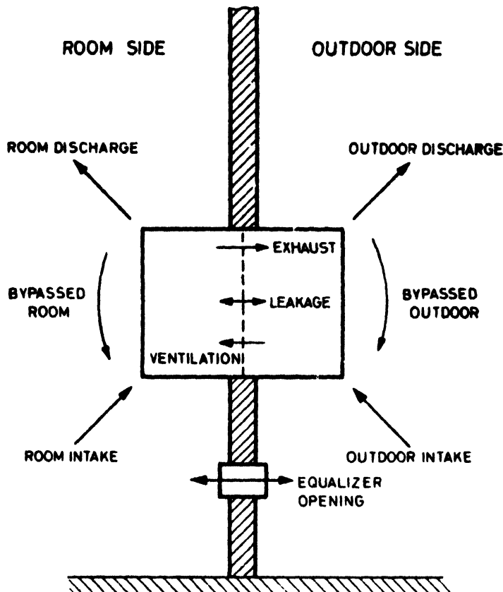
FIG. 1 DEFINITIONS RELATING TO AIR FLOW
