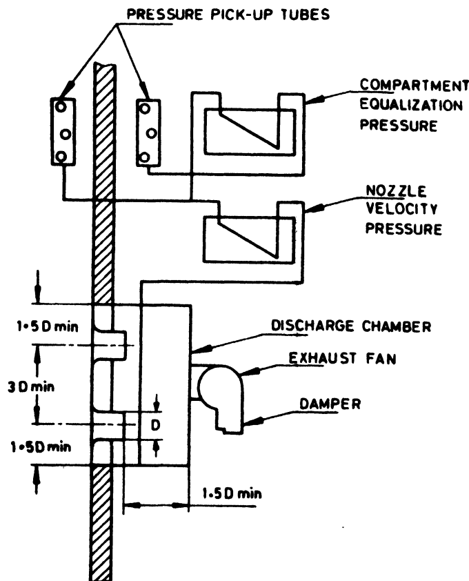
FIG. 4 PRESSURE EQUALIZING DEVICE
