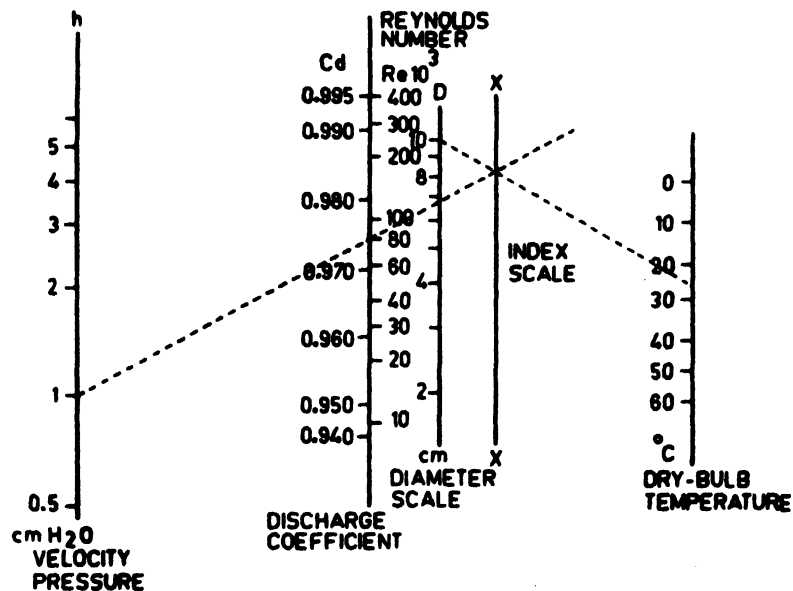
FIG. 5 DETERMINATION OF NOZZLE DISCHARGE COEFFICIENT
