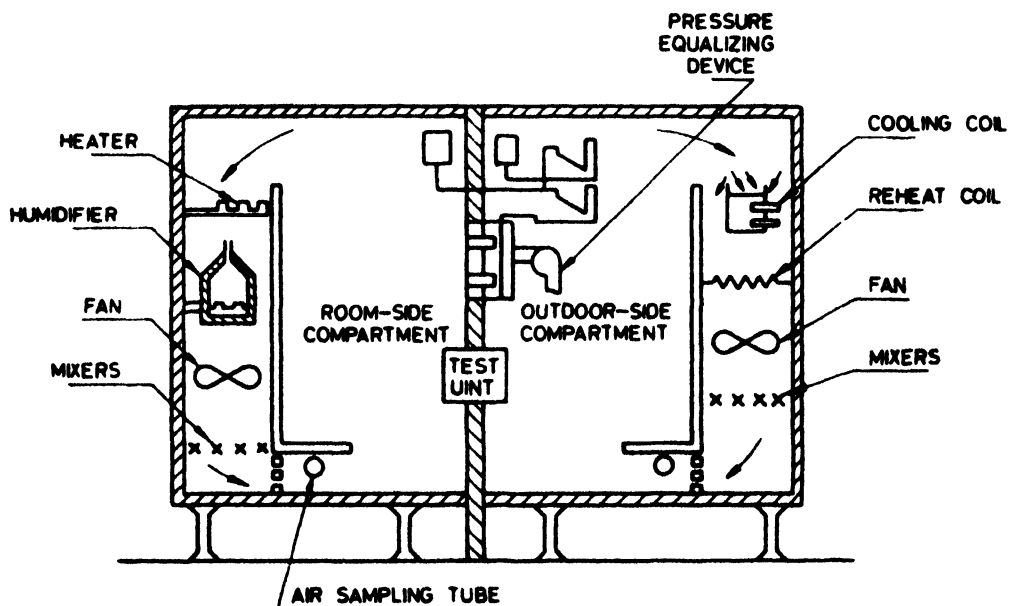
FIG. 2A CALIBRATED ROOM TYPE CALORIMETER
