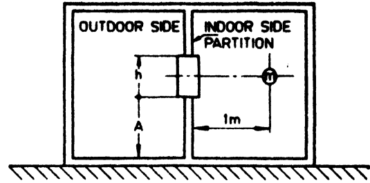
SIDE VIEW OF NOISE MEASURING ROOM
