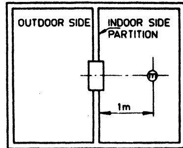
PLAN OF NOISE MEASURING ROOM
