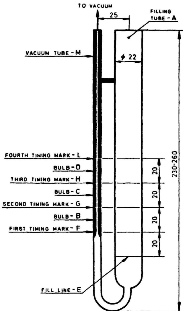
FIG. 2 ASPHALT INSTITUTE VACUUM CAPILLARY VISCOMETER
