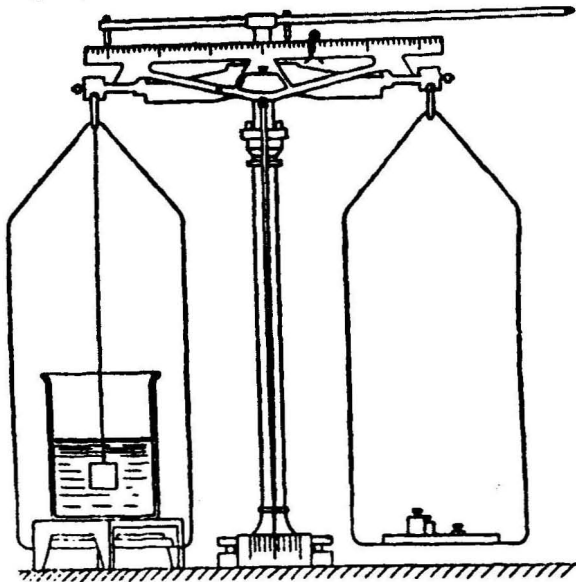
FIG. 2 ANALYTICAL BALANCE EQUIPPED WITH PAN STRADDLE
