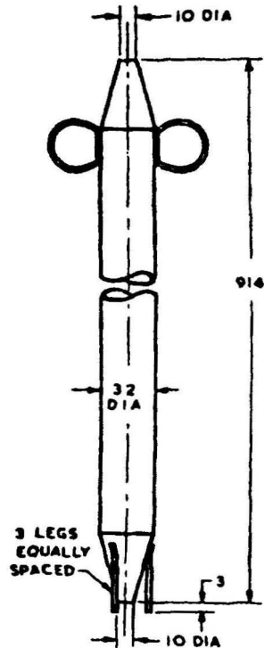
FIG. 2 SAMPLING TUBE
