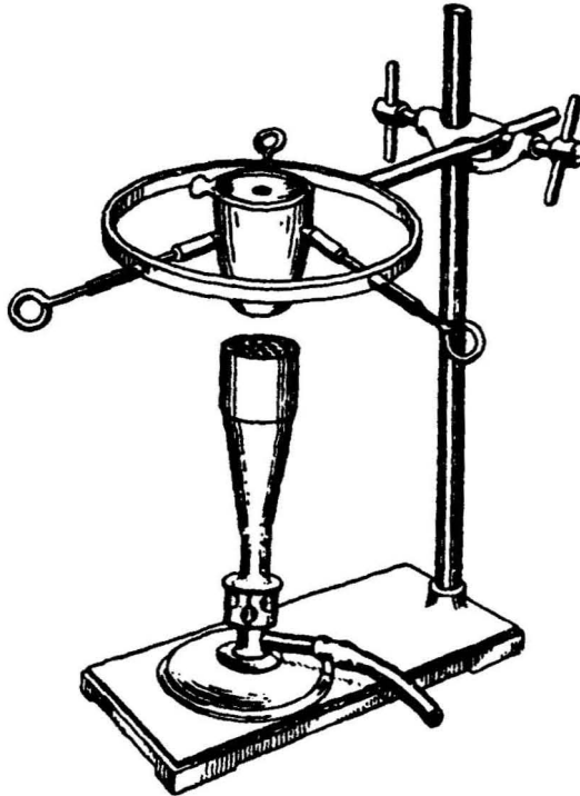
FIG. 3 ASSEMBLY OF APPARATUS
