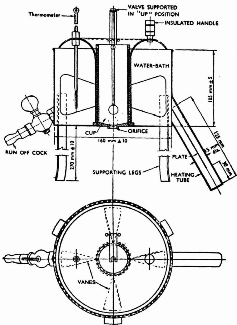
FIG. 1 TAR VISCOMETER
