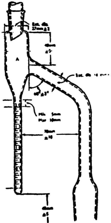
FIG. 3 2-ml RECEIVER (DEAN AND STARK APPARATUS)
