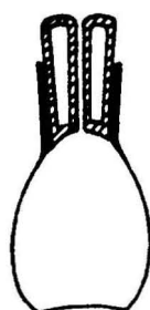
FIG. 1B WIDE-MOUTHED CAPILLARY TYPE SPECIFIC GRAVITY BOTTLE
