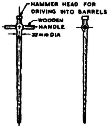
FIG. 4 SAMPLING SCOOP
