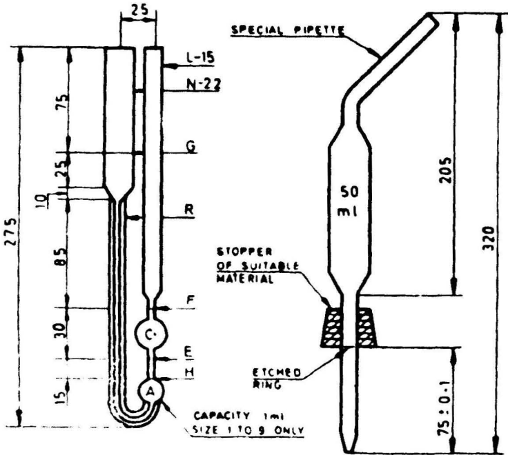
FIG. 2 BS/IP/RF U-TUBE REVERSE FLOW VISCOMETER FOR OPAQUE LIQUIDS
