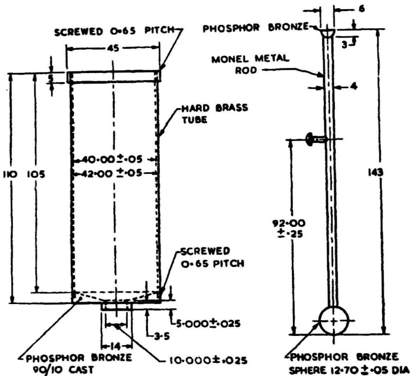
FIG. 2 10-mm TAR CUP AND VALVE
