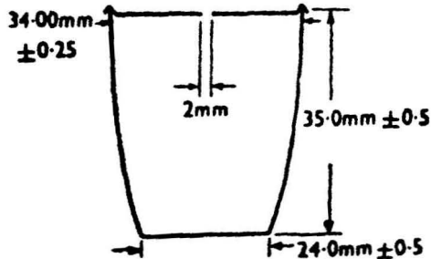
FIG. 1 PLATINUM CRUCIBLE AND LID
