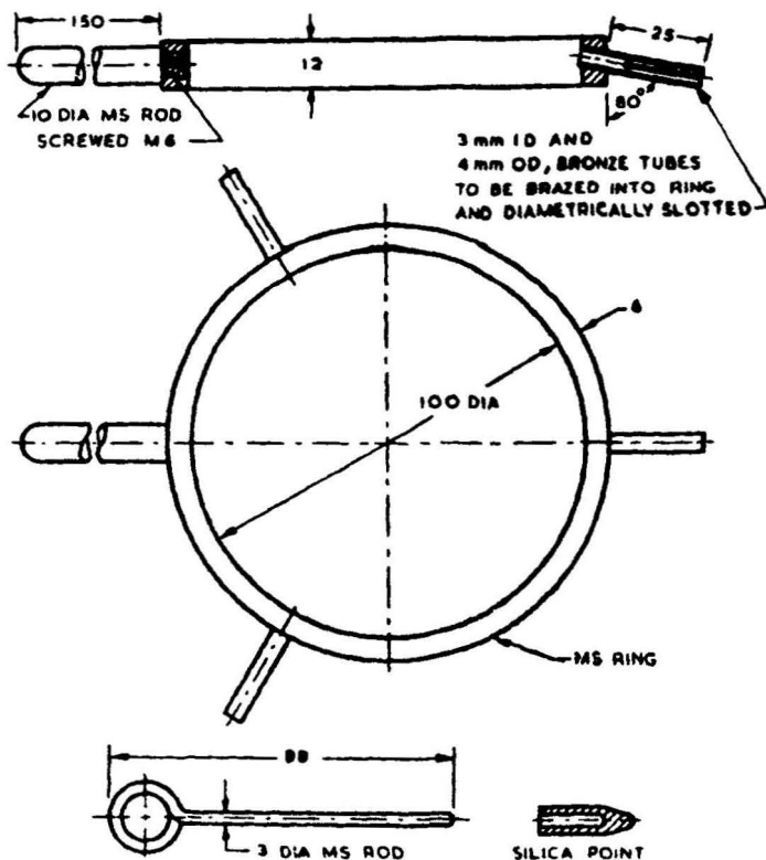
FIG. 2 THREE-ARM CRUCIBLE SUPPORT WITH SILICA POINTS
