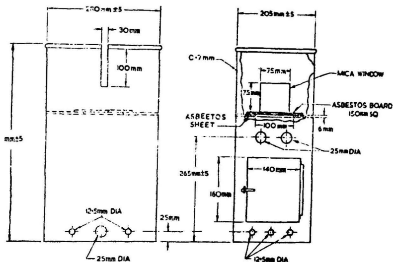
FIG. 5 DRAUGHT SCREEN
