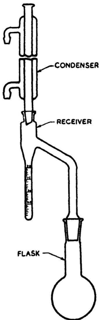
FIG. 1 DEAN AND STARK ASSEMBLY
