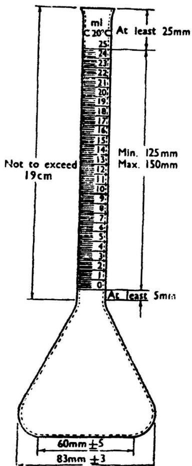
FIG. 1 PHENOLS FLASK
