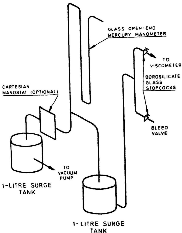
FIG. 4 SUGGESTED VACUUM SYSTEM FOR VACUUM CAPILLARY VISCOMETERS
