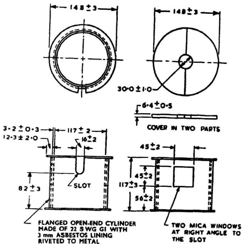
FIG. 3 SHIELD
