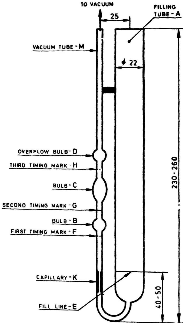
FIG. 1 CANNON-MANNING VACUUM CAPILLARY VISCOMETER
